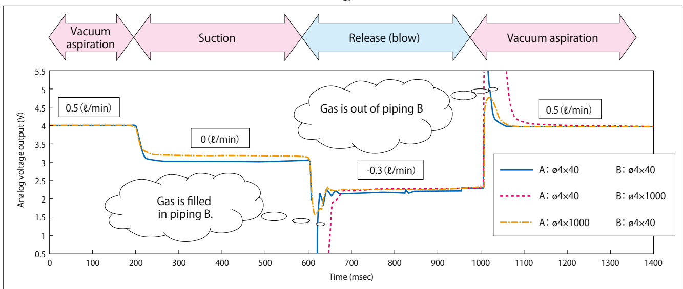
Dependence of response time on piping
