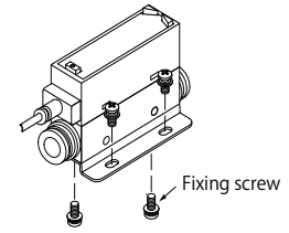
Bracket installation
