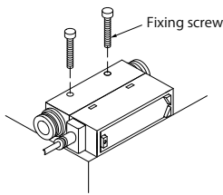
Horizontal (through hole)
