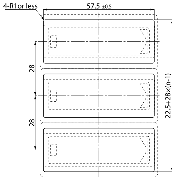
■ Side-by-side installation
